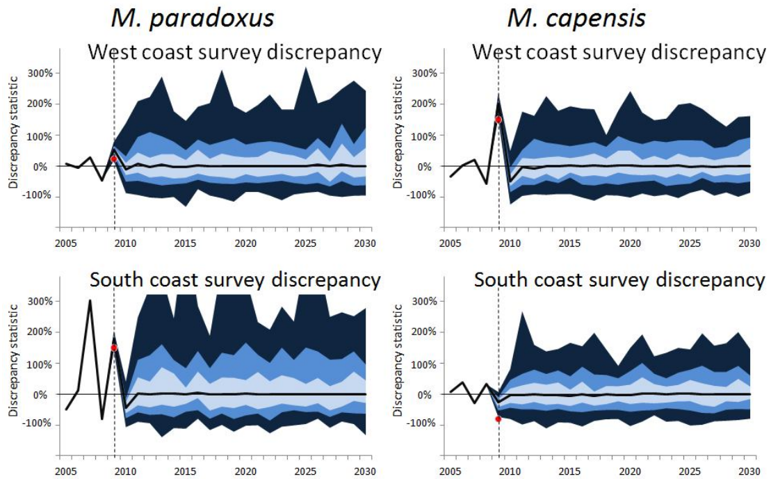
Fig. E4: 95, 75, 50% PI and median for the discrepancy statistic for M. paradoxus and M. capensis for RSa under OMP-2010.
