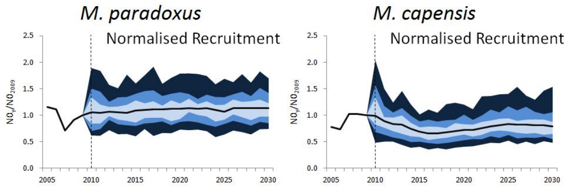
Fig. E3: 95, 75, 50% PI and median for the normalised recruitment ( N_{0y}/N_{02009} ) for M. paradoxus and M. capensis for RS1 under OMP-2010.
