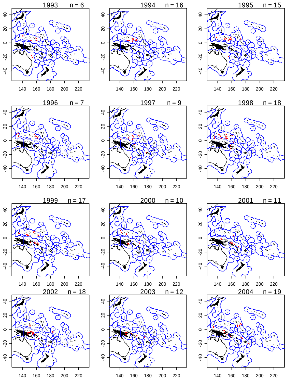
Figure 7a. Position of observed longline sets in which one or more turtles were captured in the WCPO, 1989–2004, excluding sets south of 31°S and observed sets on US vessels within and north-east of the Hawaiian EEZ. Source: observer longline data held by SPC. Missing years indicate that no turtles were observed captured from longline sets in that year.
