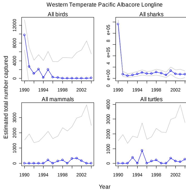
Figure 14a. Estimated total catches (numbers, blue lines) of each major taxa by the temperate Pacific albacore longline fishery, 1990–2004. Source: observer database maintained by SPC. Grey lines represent \pm two times the global standard deviations for each taxa.
