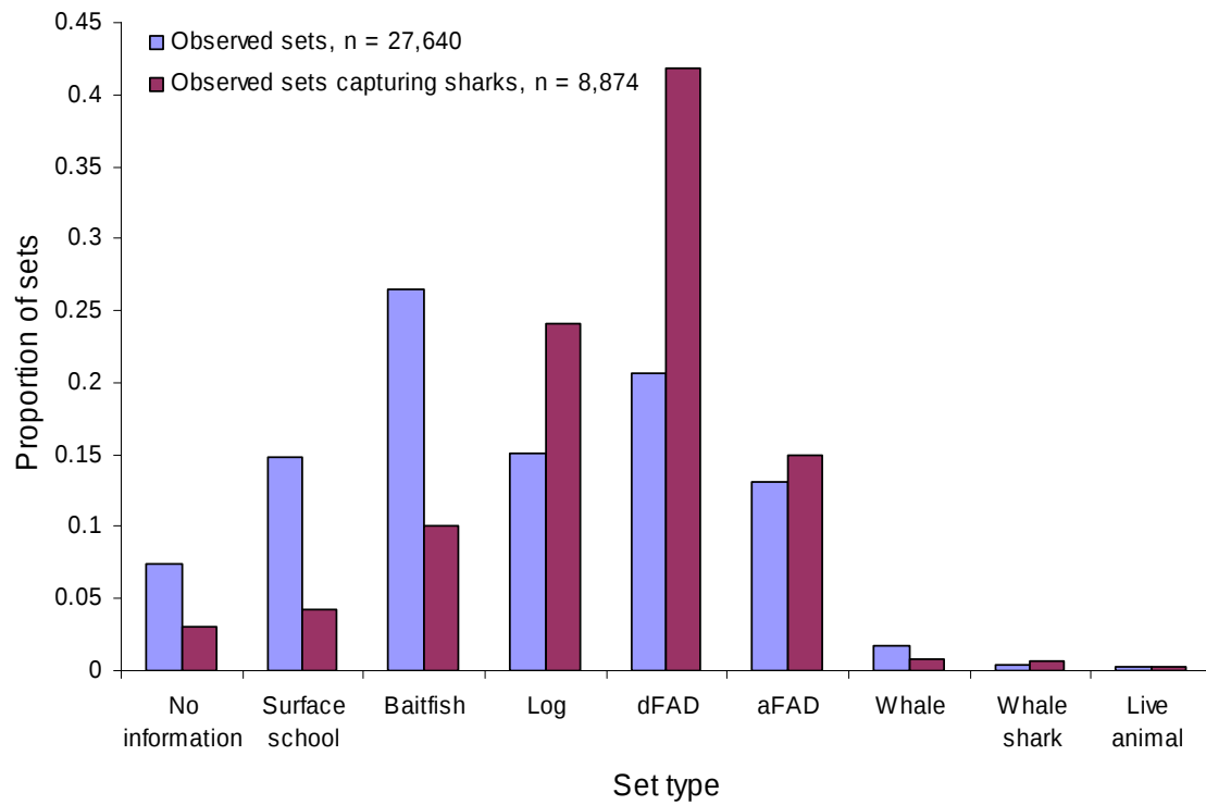
Figure 26. Distribution of the set types of observed purse-seine sets and observed purse-seine sets in which one or more sharks were captured by all fleets in the WCPO, 1994–2004. Upper figure, individual set types. Lower figure, pooled set types. Source, observer data held by SPC.
