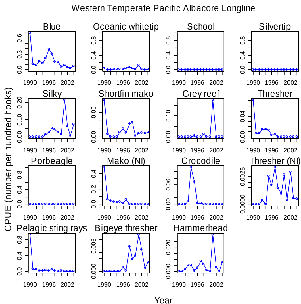
Figure 17. Estimated catch per unit effort (number per hundred hooks) of common shark taxa by the temperate Pacific albacore longline fishery, 1990–2004. Source: observer database maintained by SPC. (NI), indicates an taxa not identified to species level.
