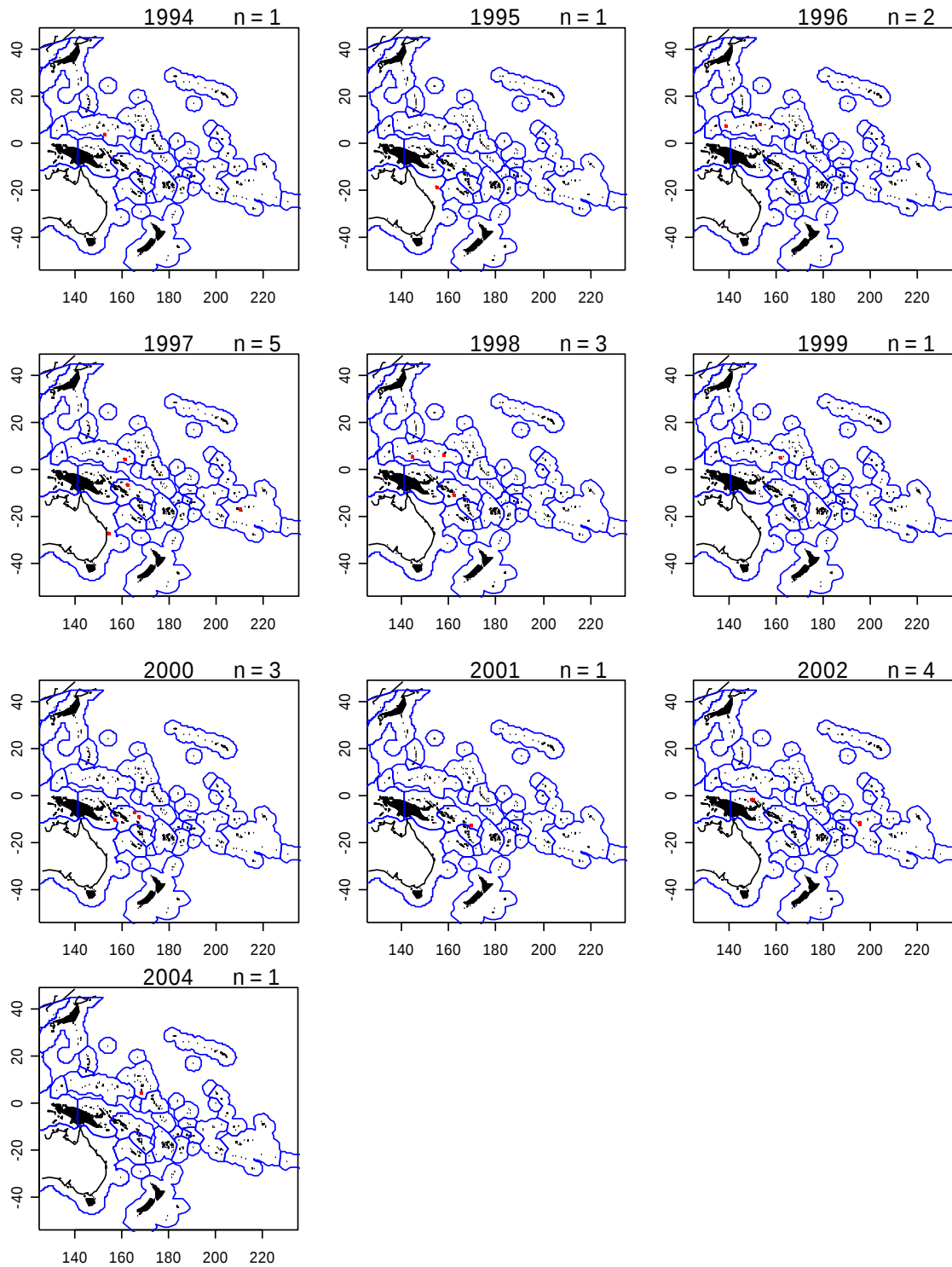
Figure 5a. Position of observed longline sets in which one or more mammals were captured in the WCPO, 1989–2004, excluding sets south of 31°S and observed sets on US vessels within and north-east of the Hawaiian EEZ. Source: observer longline data held by SPC. Missing years indicate that no mammals were observed captured from longline sets in that year.
