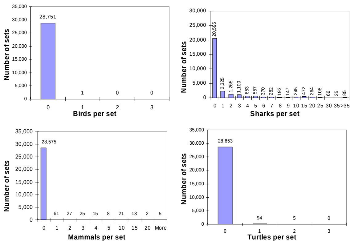
Figure 8d. Frequency of occurrence of major taxa in sets by the purse-seine fishery of the tropical western Pacific, 1994–2004. Source: observer database maintained by SPC. Total numbers of sets for each frequency category are provided above each bar.
