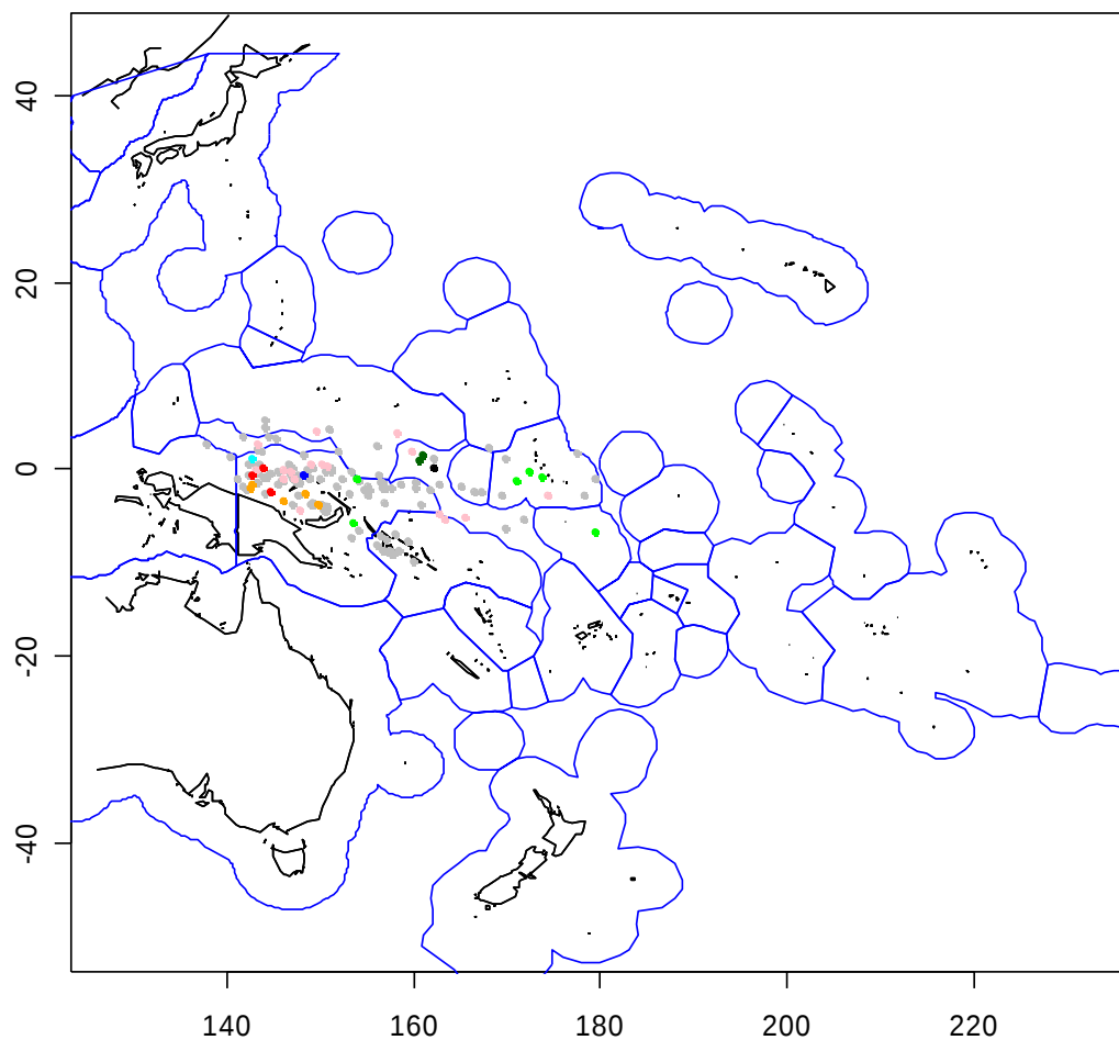
Figure 5b. Position of observed purse-seine sets in which one or more mammals were captured in the WCPO, 1995–2004. Source: observer longline data held by SPC. Codes: grey, marine mammal (unidentified); pink, dolphins/porpoises (unidentified); orange, common dolphin; red, bottlenose dolphin; green, whale (unidentified); dark blue, toothed whales (blackfish); light blue, pygmy killer whale; dark green, short-finned pilot whale; black, spinner dolphin.
