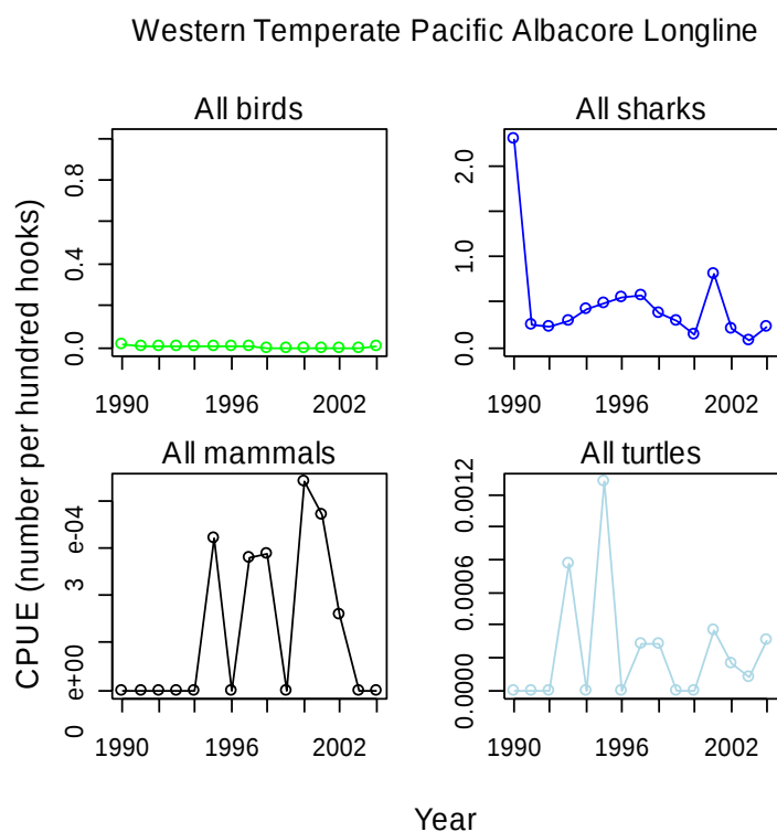
Figure 11a. Estimated catch per unit effort (number per hundred hooks) of each major taxa by the temperate Pacific albacore longline fishery, 1990–2004. Source: observer database maintained by SPC.
