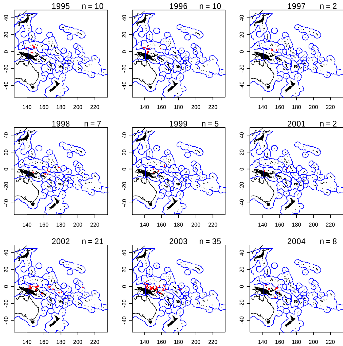
Figure 7b. Position of observed purse-seine sets in which one or more turtles were captured by all fleets in the WCPO, 1994–2004. Source: observer purse-seine data held by SPC. Missing years indicate that no turtles were observed captured from purse-seine sets in that year.
