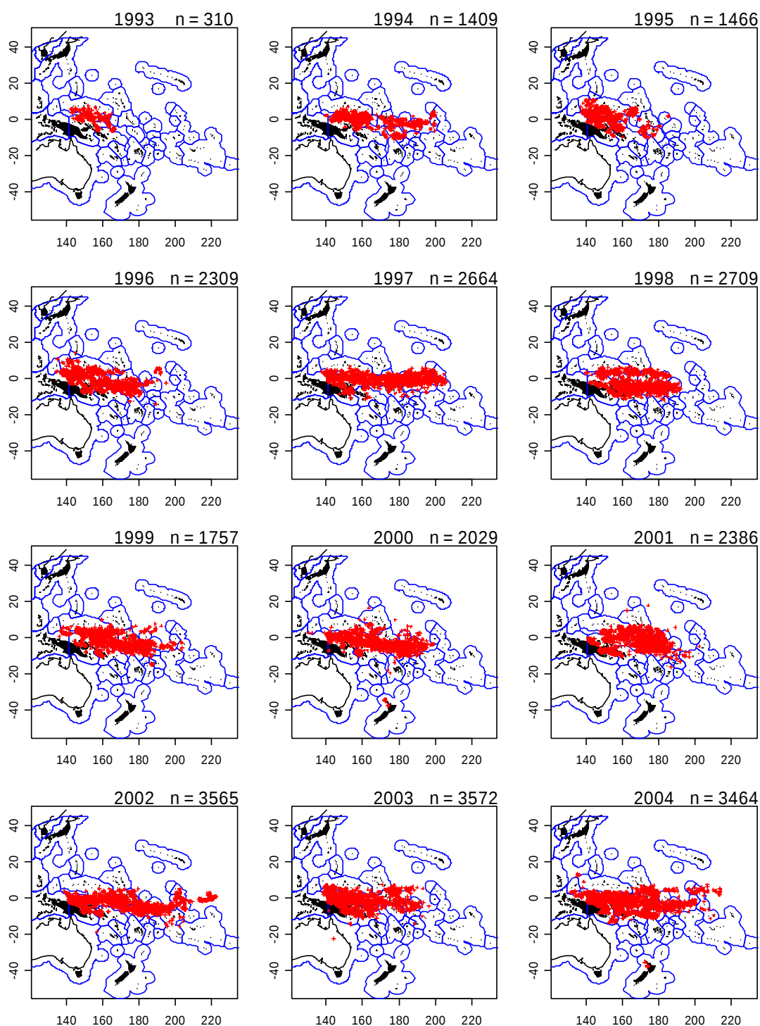
Figure 2. Position of observed purse-seine sets in the WCPO, 1993–2004. Source: observer purse-seine data held by SPC. Data for 2004 may be incomplete. n denotes the number of observed sets per year.
